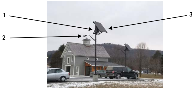
Single Solar Module Unit
